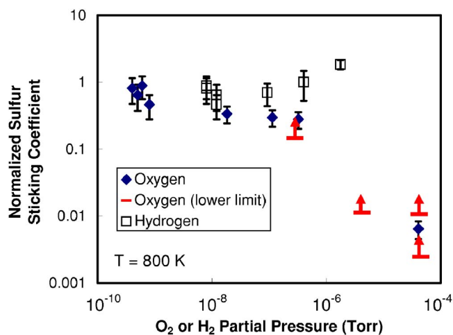
FIG. 8. (Color online) Effect of oxygen and hydrogen on the deposition of sulfur by exposure to \text{H}_2\text{S} at 527 °C. Sticking coefficient ( S adsorbed per incident \text{H}_2\text{S} molecule) of \text{H}_2\text{S} to the Pt gate in \text{O}_2 and \text{H}_2 background pressures, normalized to the value at the lowest background pressure. The horizontal bars with arrows represent lower limits; in these measurements the surface was saturated with sulfur after the \text{H}_2\text{S} exposure, as discussed in the text. Hydrogen has virtually no effect, while oxygen significantly suppresses, but does not prevent sulfur deposition. These experiments include \text{O}_2/\text{H}_2\text{S} partial pressure ratios up to \sim 20 and \text{H}_2/\text{H}_2\text{S} ratios up to \sim 600 .
